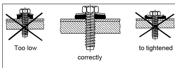
Fig. 4b: Design of screw connections (s. also IFBS assembly guidelines)
