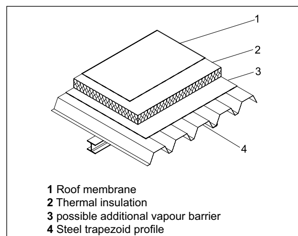
Fig. 1: Single-shell steel trapezoid profile warm roof
