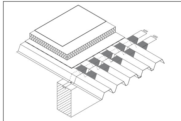
Fig. 5: Fire-stopping of the cavities
