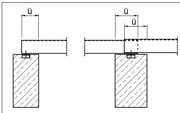
Fig. 2: Projection of the trapezoid profile panel on the support
