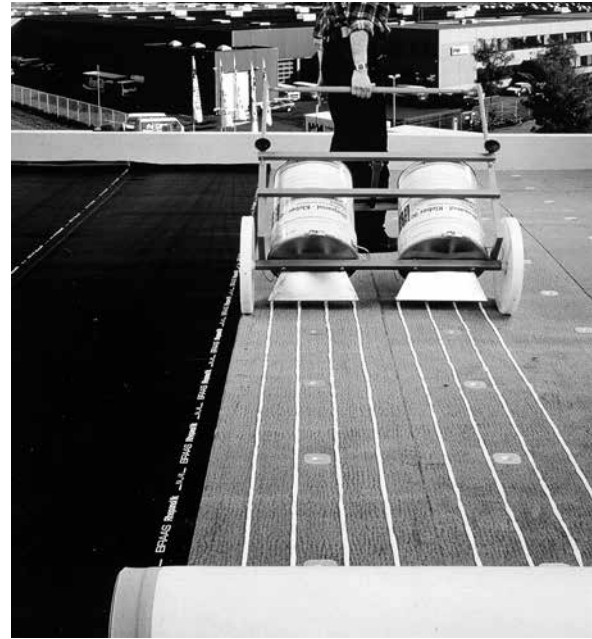
Fig. 7: Thermal insulation – adhesion
