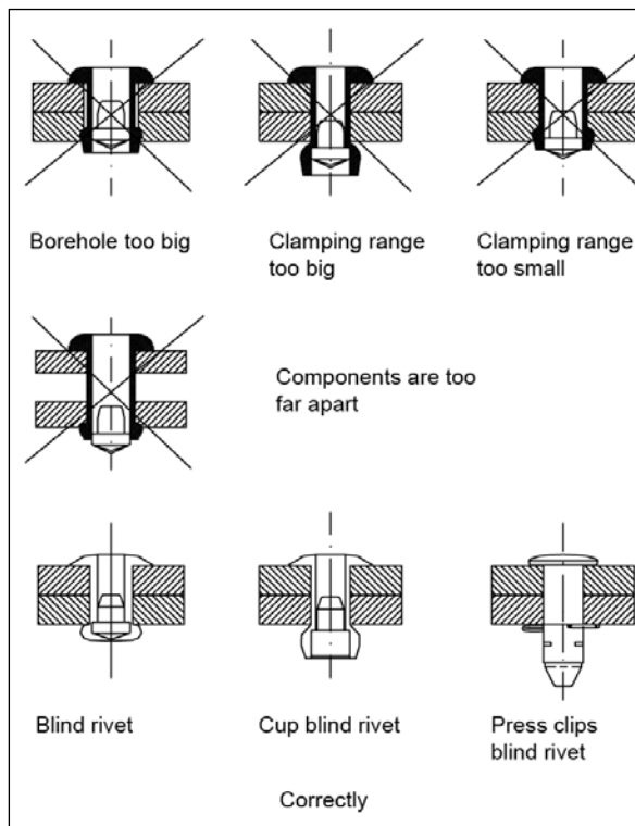
Fig. 4a: Design of rivet connections (s. also IFBS assembly guidelines)
