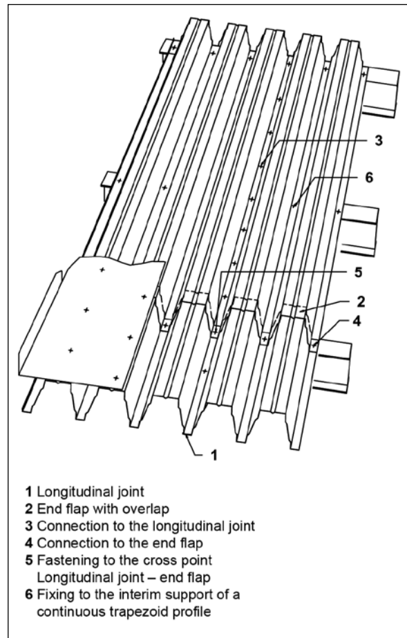
Fig. 3: Fixing in the area of the end flaps and longitudinal joints (s. also IFBS assembly guidelines)
