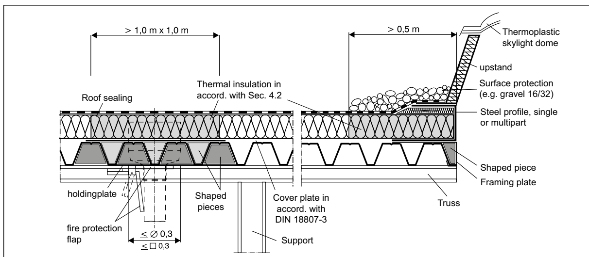
Fig. 8: Design example of a roof penetration
